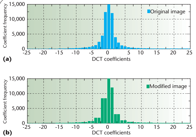
Figure 4. Frequency histograms. Sequential changes to the (a) original and (b) modified image's least-sequential bit of discrete cosine transform coefficients tend to equalize the frequency of adjacent DCT coefficients in the histograms.
